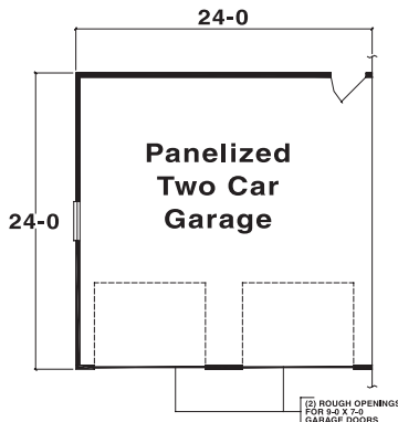
Option F Panelized Garage 24'-0" x 24'-0"
