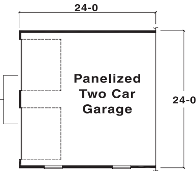
Option B Panelized Garage 24'-0" x 24'-0"
