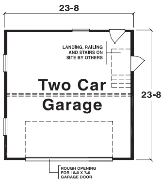
Option B Modular Garage 23'-8" x 23'-8"
