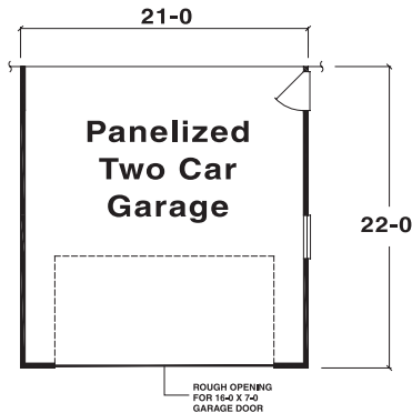
Option C Panelized Garage 21'-0" x 22'-0"
