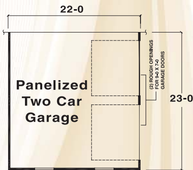
Option D Panelized Garage 22'-0" x 23'-0"
