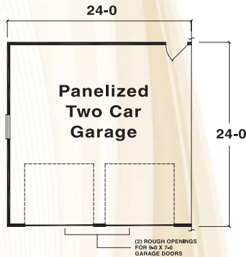
Option A Panelized Garage 24'-0" x 24'-0"
