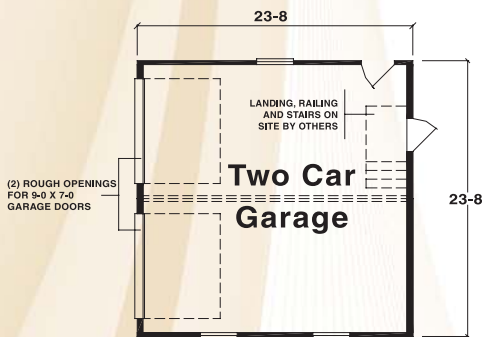
Option A Modular Garage 23'-8" x 23'-8"
