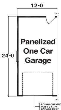
Option E Panelized Garage 12'-0" x 24'-0"
